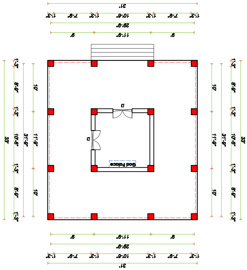
Proposed - Temple Floor Plan (Scale 1"=8'-0") Temple Area :- 1023.00 Sq.ft
